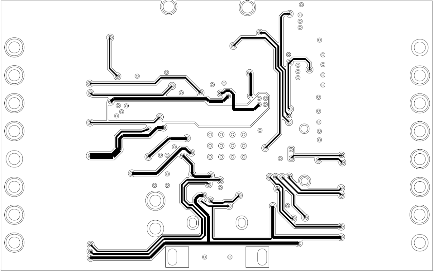
Figure 26. P9235A-R-EVK Layout (Bottom Layer)
